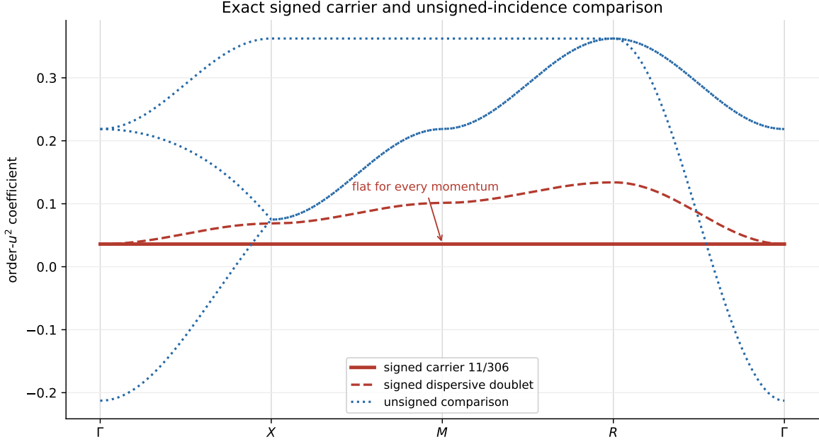
Figure 2: Order- u^2 coefficients along \Gamma - X - M - R - \Gamma . The red carrier and dispersive doublet are the signed incidence result; their conditional global assembly is Corollary 11. The blue curves are the exact unsigned-incidence comparison spectrum. Reading the blue curves as physical charge-even bands requires the separate symbol hypothesis of Section 6.
