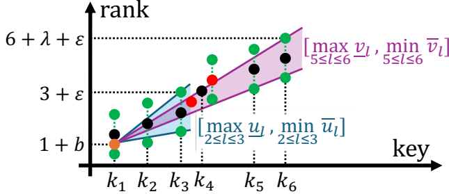
Figure 16: An example of DI-CONSECUTIVE evaluating a candidate poison sequence (starting from k_3 + 1 with \lambda = 2 ). For a specific intercept b , slope ranges for pre-poison ( k_2, k_3 ) and post-poison ( k_5, k_6 ) keys are retrieved in O(1) via sparse tables. The slope range for the poisons is also computed in O(1) by finding the range covering k_3 + 1 and the largest poison.
