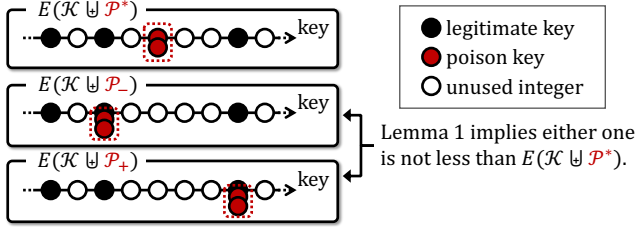
Figure 12: Step 2 of the proof of Theorem 2: showing \text{Supp}(\mathcal{P}^*) \subseteq \mathcal{K} . By shifting a block in \text{Supp}(\mathcal{P}^*) \setminus \mathcal{K} left or right, we can reduce |\text{Supp}(\mathcal{P}^*) \setminus \mathcal{K}| without decreasing the objective.
