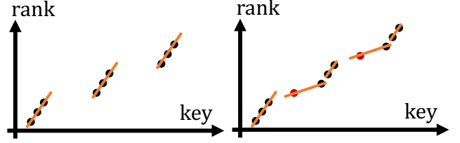
Figure 15: An example of the tight upper bound (Theorem 6), where \lambda = 2 and \varepsilon = 0 . Before poisoning (left), m_{\text{opt}}(\mathcal{K}, \varepsilon) = 3 and after poisoning (right), m_{\text{opt}}(\mathcal{K} \cup \mathcal{P}, \varepsilon) = 5 .
