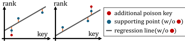
Figure 11: Step 1 of the proof of Theorem 2: showing |\mathcal{P}^*| = \lambda . Regardless of how the three supporting points are arranged, we can always add a suitable poison to strictly increase the maximum error.
