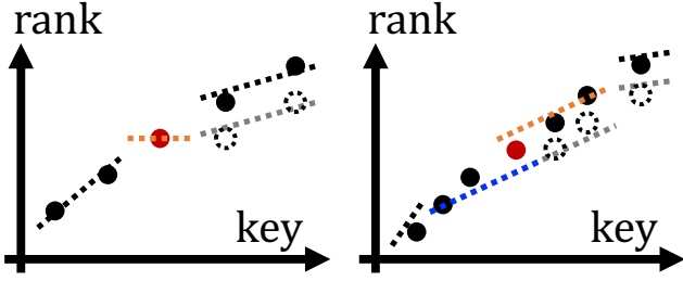
Figure 14: Proof of Theorem 5. (1) Case 1 (left): when p lies between two adjacent segments, we add a new segment covering only p . (2) Case 2 (right): when p lies inside an existing segment, we split the segment containing p into two.
