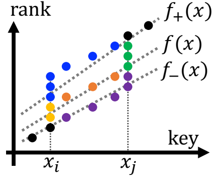
Figure 13: Step 3 of the proof of Theorem 2. The figure illustrates the case where d_i = 2 and d_j = 3 . Property 1 shows that the error of f with respect to the black, yellow, and green points is at most \varepsilon . Property 2 shows that the error for the orange points is at most \varepsilon .
