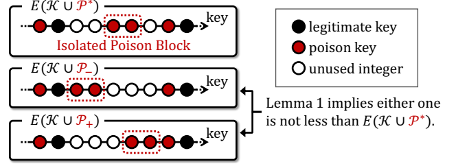
Figure 10: Illustration of the proof of Theorem 1. By Lemma 1, shifting an isolated poison block can reduce the number of isolated poison blocks without decreasing the maximum error.
