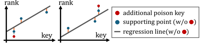
Figure 10: Step 1 of the proof of Theorem 2: showing |\mathcal{P}^*| = \lambda . Regardless of how the three supporting points are arranged, we can always add a suitable poison to strictly increase the maximum error.
