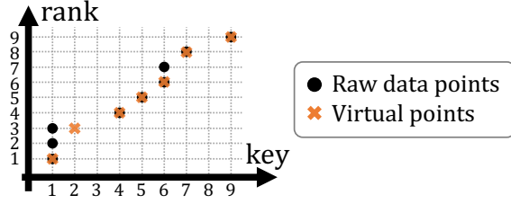
Figure 21: PLA construction with duplicate keys in the PGM-index. Instead of directly constructing the PLA from the original key-rank pairs, the PGM-index constructs the PLA over a set of virtual points introduced to handle duplicates.
