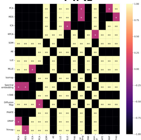
ARI
