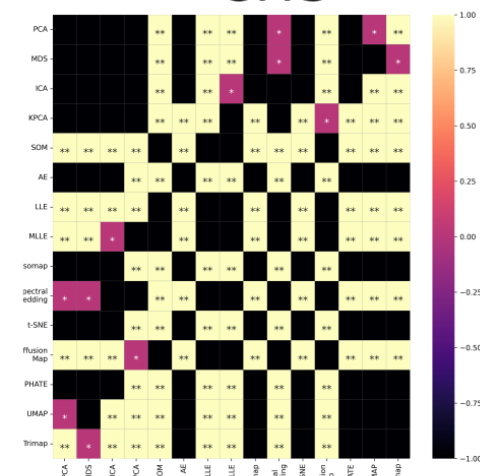
CHS
