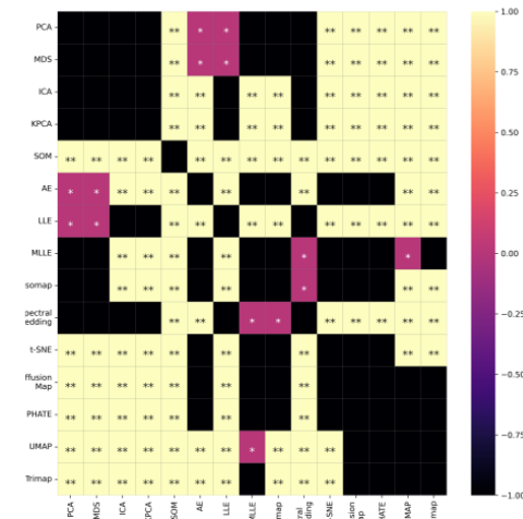
SS
