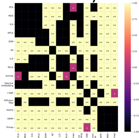
Purity
