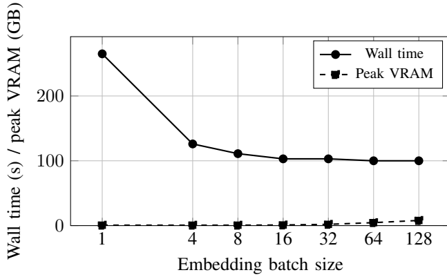
Fig. 8. Throughput and peak-VRAM vs. embedding batch size at fp32 on the 2.2 h reference file (RTX A6000). Wall time saturates by batch 16; peak VRAM grows linearly above batch 8.
