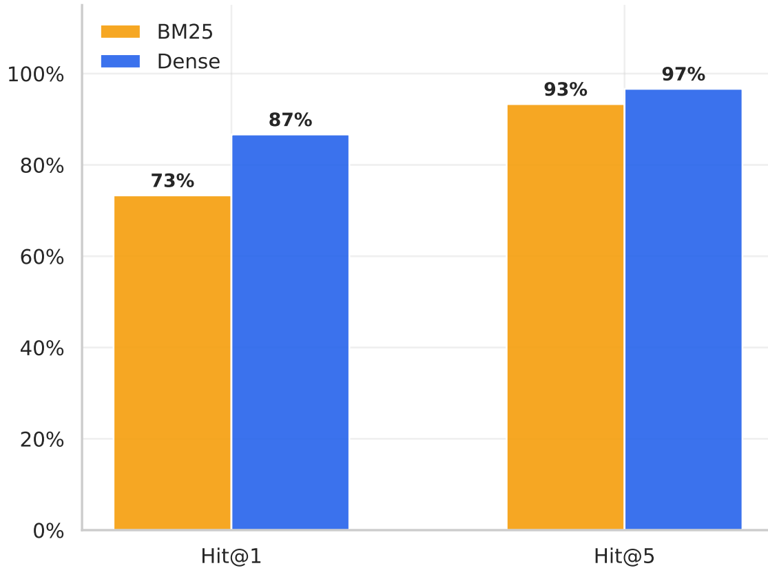
BM25 vs Dense Retrieval (Hit@1 and Hit@5)
