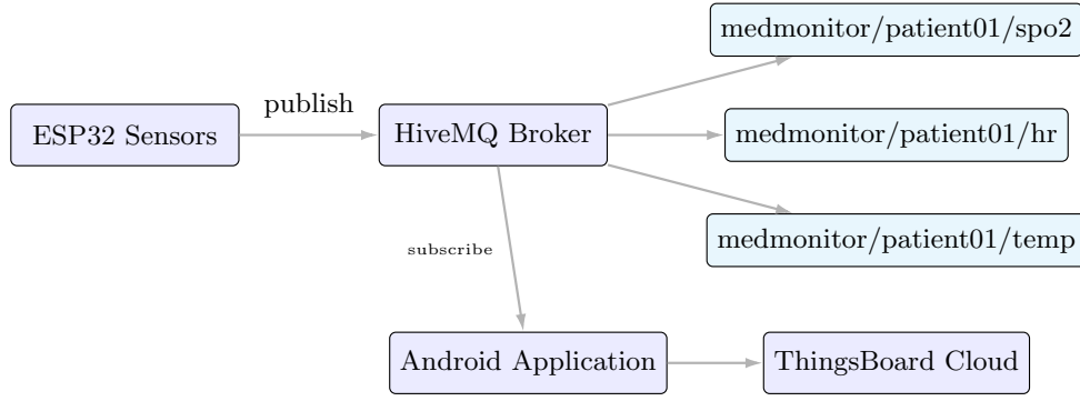
Fig. 5 MQTT topic hierarchy for the Android companion application: per-vital topics on a HiveMQ broker, subscribed to by the mobile app.
