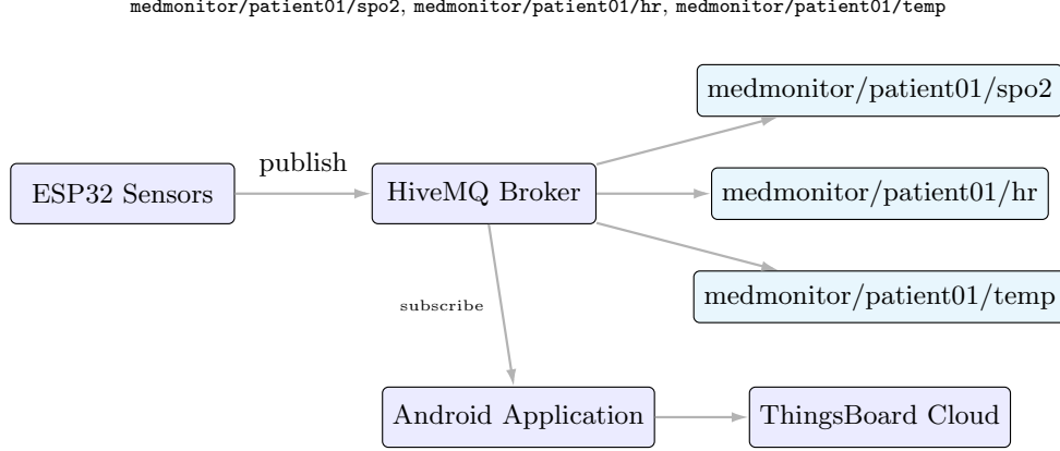
Fig. 5 MQTT topic hierarchy for the Android companion application: per-vital topics on a HiveMQ broker, subscribed to by the mobile app.
