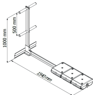
Support Eco-Stable T19 droit
