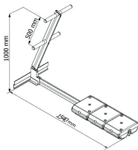
Support Eco-Stable T19 incliné 22°
