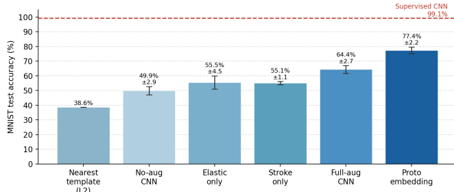
Figure 3: MNIST test accuracy for all one-shot configurations. Error bars show \pm 1 standard deviation across seeds. Dashed line: supervised CNN reference (99.11%).
