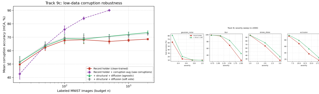
Figure 3: Left: mean corruption accuracy vs. budget—the agnostic ensemble ( conf_all ) beats the clean-trained record holder everywhere; informed augmentation ( record_aug ) is stronger once \geq 100 labels are available. Right: severity sweep at n = 2000 —the advantage grows with severity, except under destructive noise.
