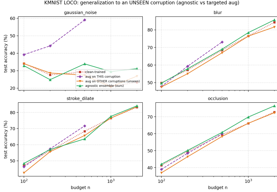
Figure 2: KMIST leave-one-corruption-out. The agnostic ensemble (green) matches or beats augmentation trained on the other corruptions (orange) on all four types for n \geq 1000 .
