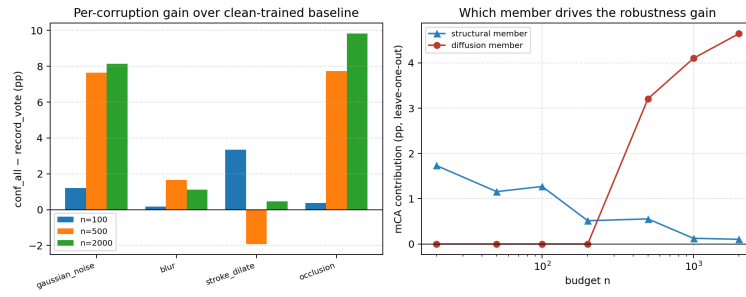
Figure 4: Left: per-corruption gain of conf_all over the clean-trained baseline. Right: leave-one-member-out mCA contribution—structural at low n , diffusion at n \geq 500 .
