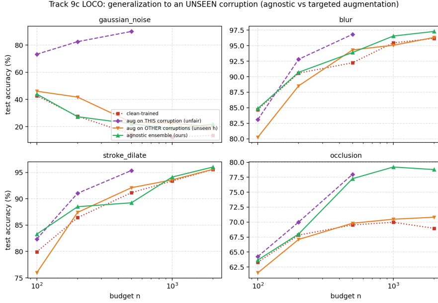
Figure 1: Leave-one-corruption-out (MNIST). On blur, stroke thickening and occlusion the corruption-agnostic ensemble (green) matches or beats augmentation trained on the other corruptions (orange) at the unseen corruption; gaussian noise is the exception.
