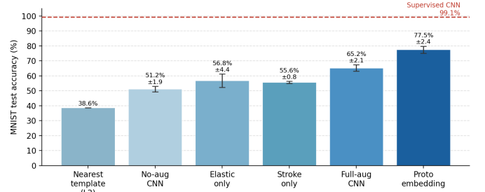
Fig. 3. MNIST test accuracy for all one-shot configurations. Error bars show \pm 1 standard deviation across seeds. Dashed line: supervised CNN reference (99.11%).
