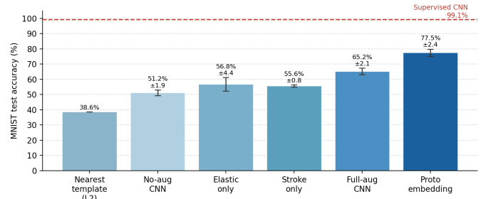
Fig. 3. MNIST test accuracy for all one-shot configurations. Error bars show \pm 1 standard deviation across seeds. Dashed line: supervised CNN reference (99.1%).
