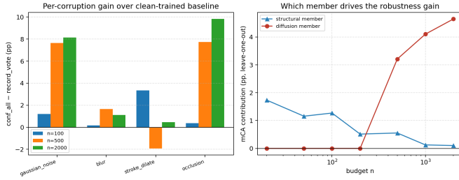
Fig. 3. Left: per-corruption gain of \text{conf\_all} over the clean-trained baseline. Right: leave-one-member-out mCA contribution—structural at low n , diffusion at n \geq 500 .
