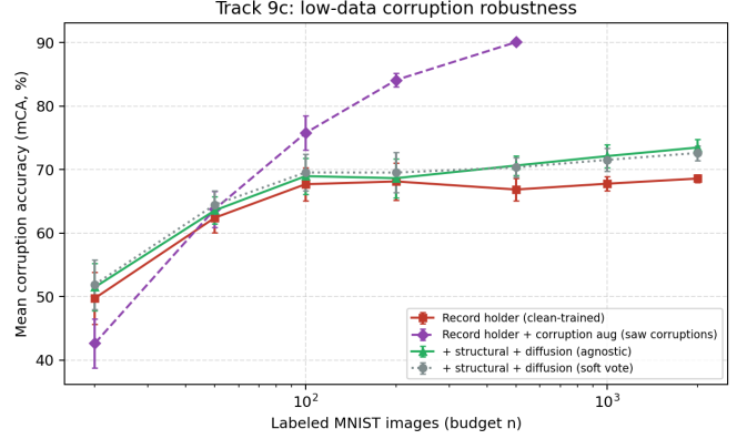
Fig. 1. Mean corruption accuracy versus labelled budget. The agnostic ensemble ( conf_all ) beats the clean-trained record holder everywhere; informed augmentation ( record_aug , dashed) is stronger once \geq 100 labels are available.
