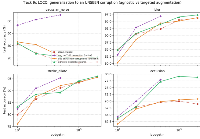
Fig. 2. Leave-one-corruption-out. On blur, stroke thickening and occlusion the corruption-agnostic ensemble (green) matches or beats augmentation trained on the other corruptions (orange) at the unseen corruption; gaussian noise is the exception.
