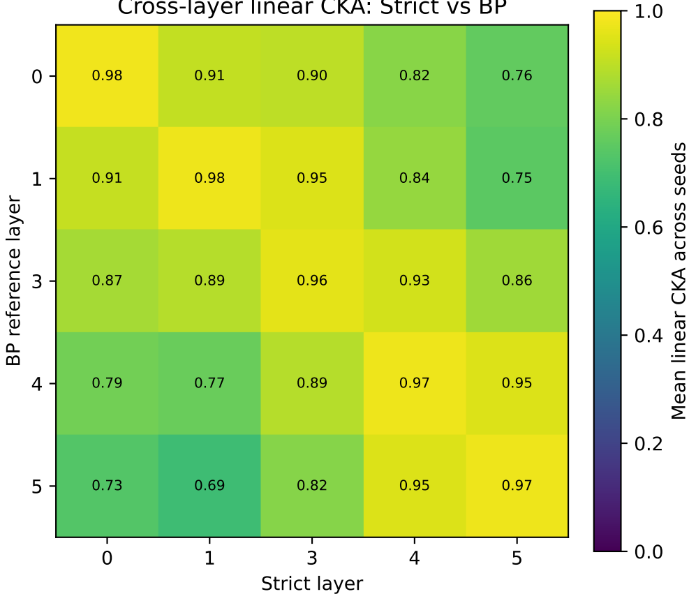
Cross-layer linear CKA: Strict vs BP
