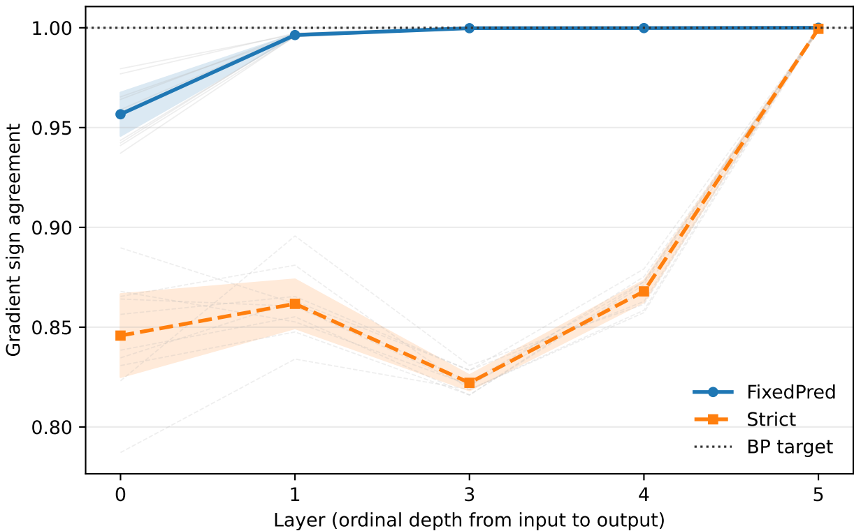
Gradient sign agreement
