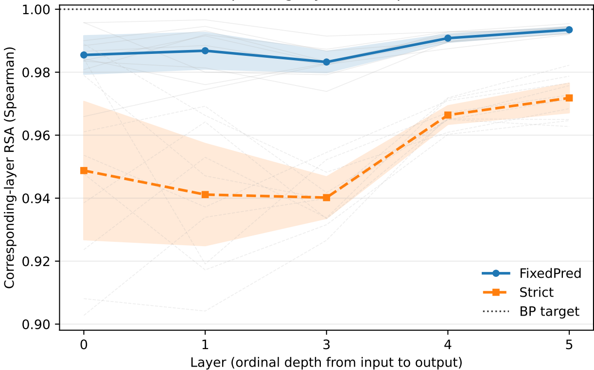
Corresponding-layer RSA (Spearman)
