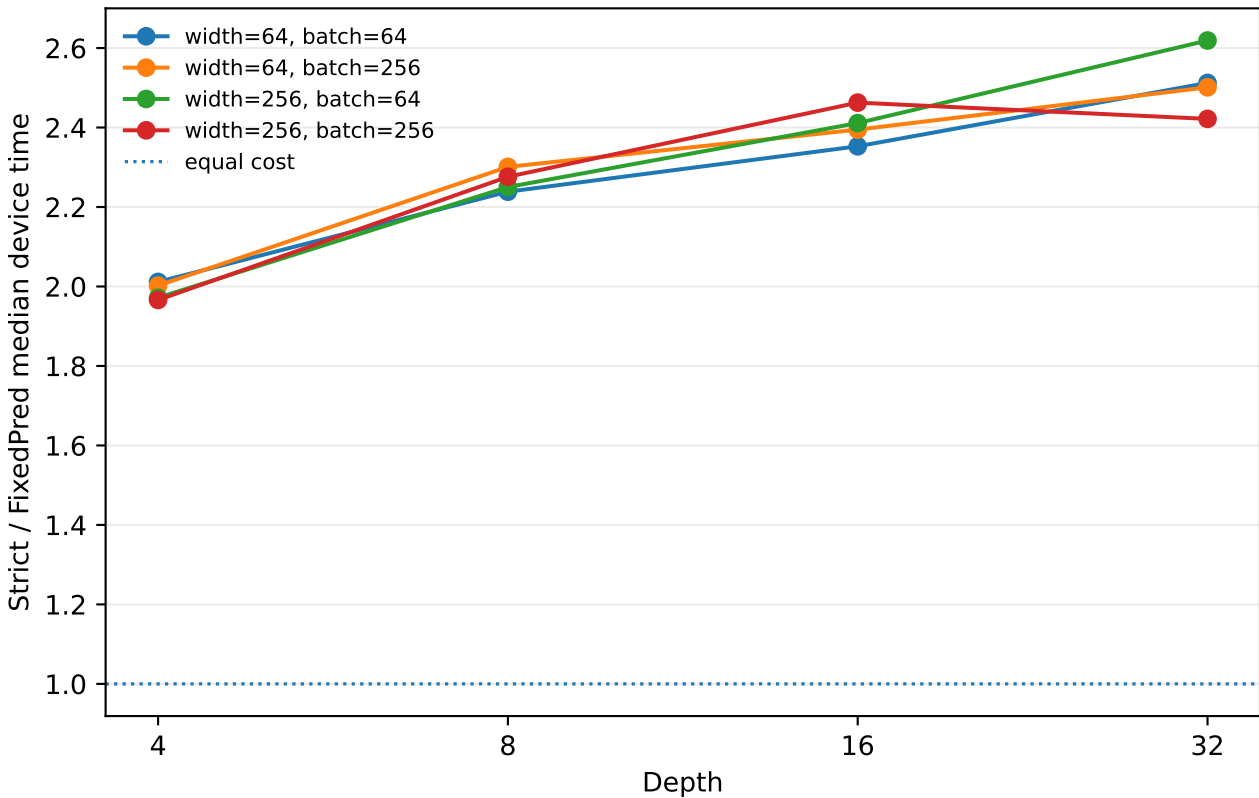
Strict relative to FixedPred: device time
