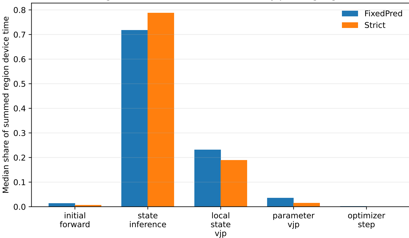
Stage 3B B0 device-time attribution by profiling region
