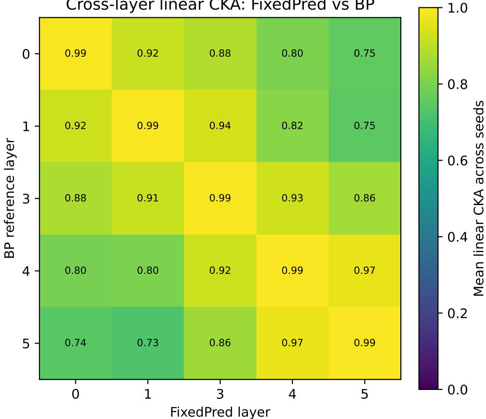
Cross-layer linear CKA: FixedPred vs BP
