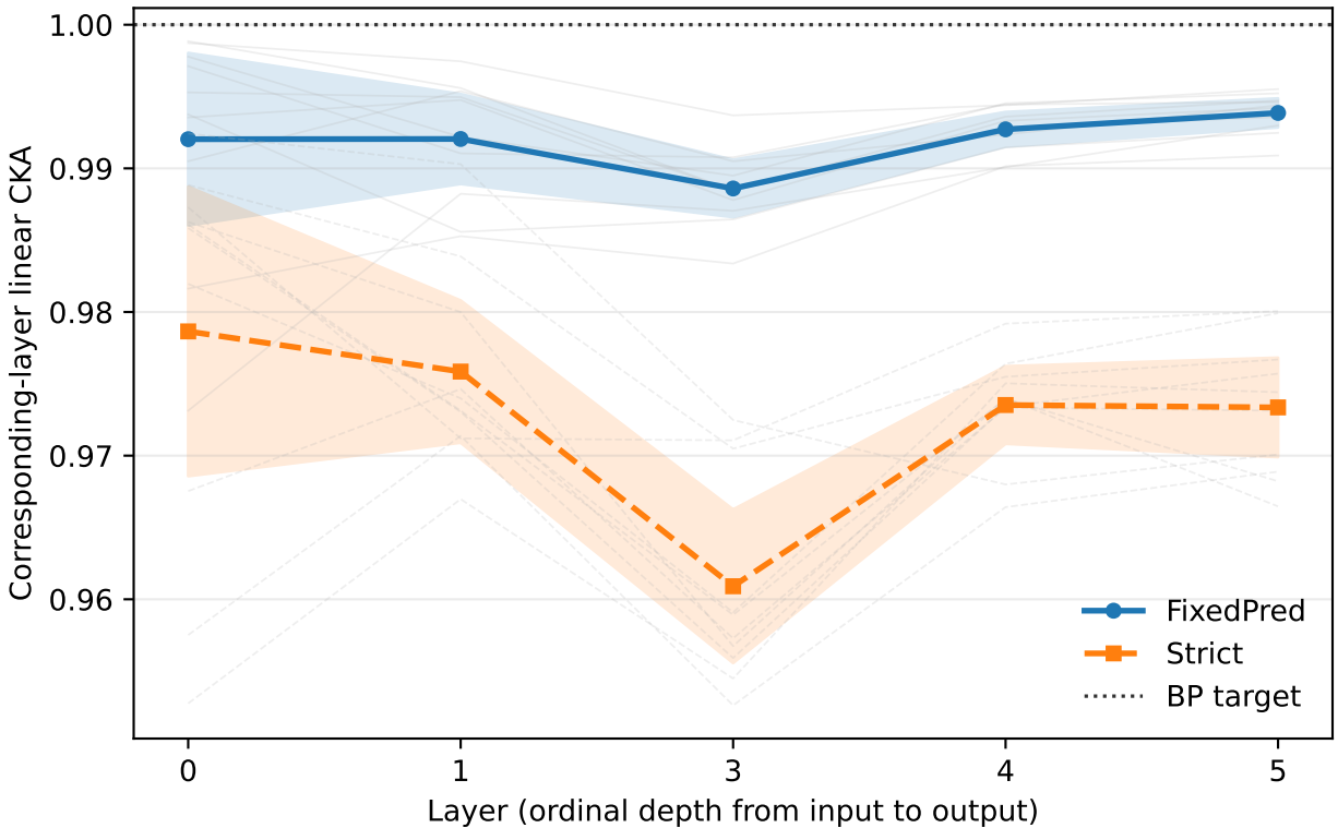
Corresponding-layer linear CKA
