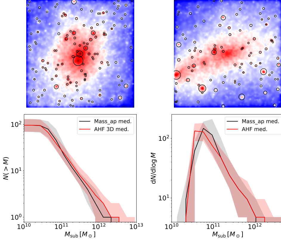
Fig. 1: Validation of the adaptive aperture algorithm. Top panels: two representative projected mass maps with adaptive apertures overlaid as black circles when the subhalos are known a priori. Bottom-left: cumulative subhalo mass function N(>M) computed from the 2D aperture masses (grey envelope and black median), compared to the 3D AHF catalogue masses (red envelope and red median), both shown as the 16th–84th percentile range across all 3273 simulated clusters. Bottom-right: corresponding differential subhalo mass function.
