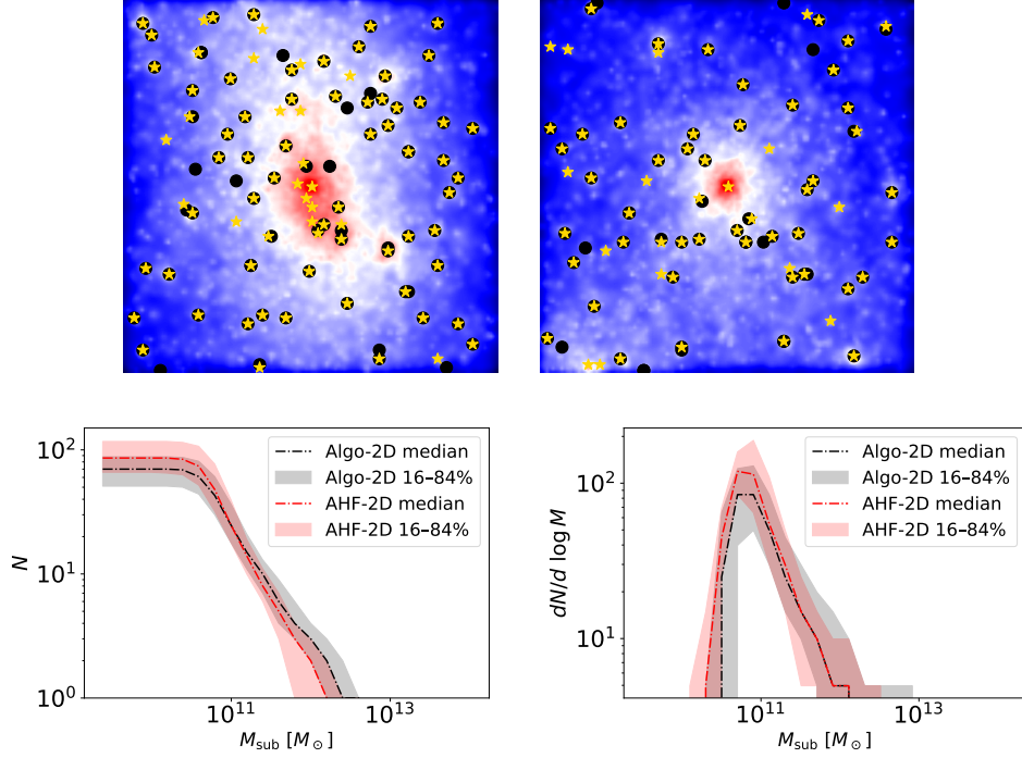
Fig. 2: Subhalo peak detection algorithm performance Top panels: two representative projected mass maps from the test set, with true AHF subhalo positions marked as black circles and algorithm-detected peaks as gold stars. The algorithm recovers the majority of true subhalo positions, including substructures in the outskirts of the cluster, with only a small number of missed detections and false positives. Bottom-left: cumulative subhalo mass function computed from the aperture masses of the algorithm-detected peaks (black, Algo-2D) and the true AHF peaks (red, AHF-2D), shown as the median and 16th–84th percentile range across the full simulation sample. Bottom-right: corresponding differential subhalo mass function.
