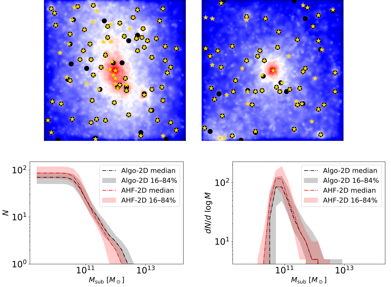
Fig. D.2: Subhalo peak detection algorithm performance Top panels: two representative projected mass maps from the test set, with true AHF subhalo positions marked as black circles and algorithm-detected peaks as gold stars. The algorithm recovers the majority of true subhalo positions, including substructures in the outskirts of the cluster, with only a small number of missed detections and false positives. Bottom-left: cumulative subhalo mass function computed from the aperture masses of the algorithm-detected peaks (black, Algo-2D) and the true AHF peaks (red, AHF-2D), shown as the median and 16th–84th percentile range across the full simulation sample. Bottom-right: corresponding differential subhalo mass function.
