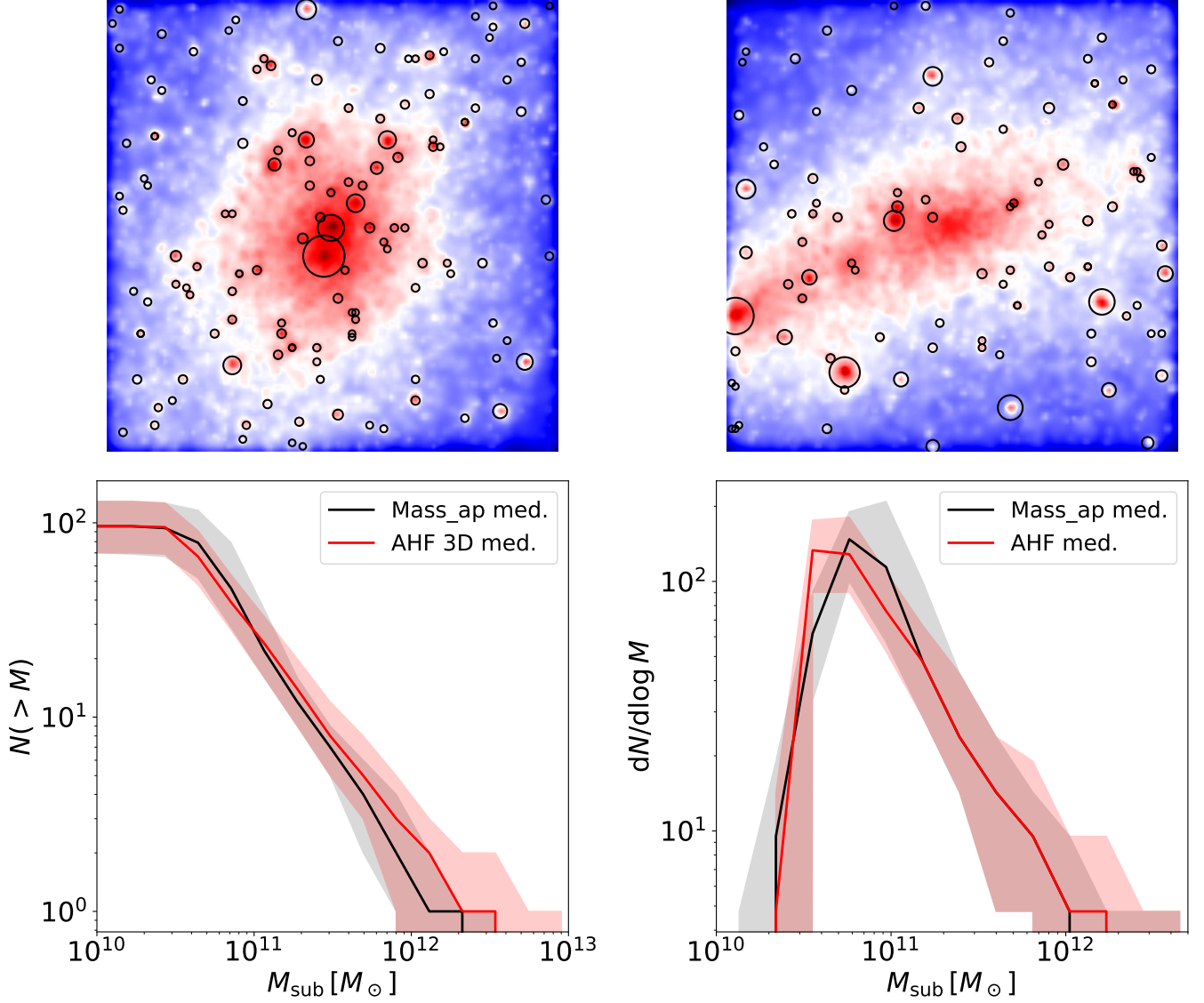
Fig. D.1: Validation of the adaptive aperture algorithm. Top panels: two representative projected mass maps with adaptive apertures overlaid as black circles when the subhalos are known a priori. Bottom-left: cumulative subhalo mass function N(> M) computed from the 2D aperture masses (grey envelope and black median), compared to the 3D AHF catalog masses (red envelope and red median), both shown as the 16th–84th percentile range across all 3273 simulated clusters. Bottom-right: corresponding differential subhalo mass function.
