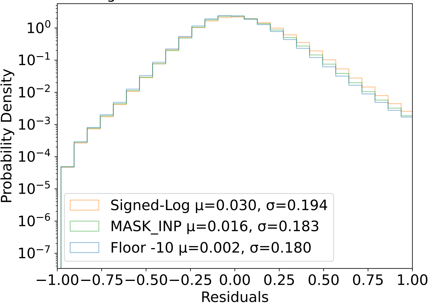
Histogram of Relative Errors for Multi-Encoder
