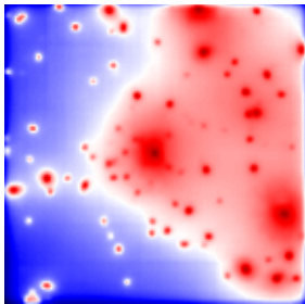
F625w
