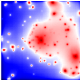
F775w
