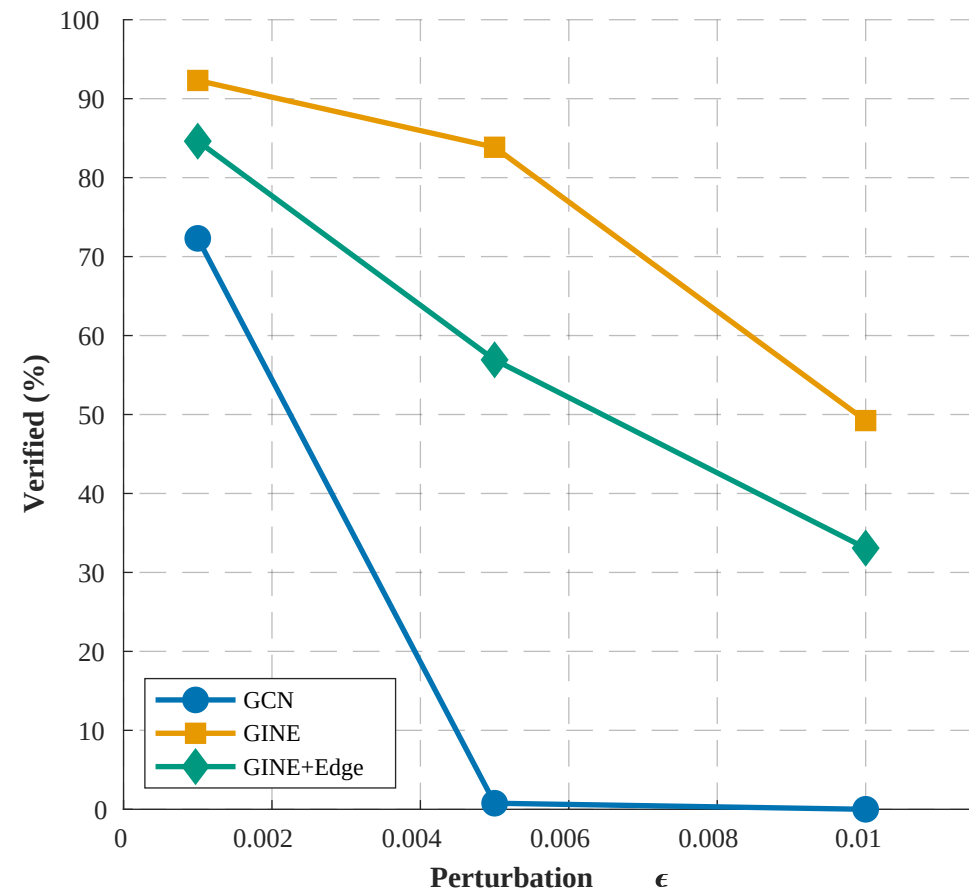
Verification vs. Perturbation
