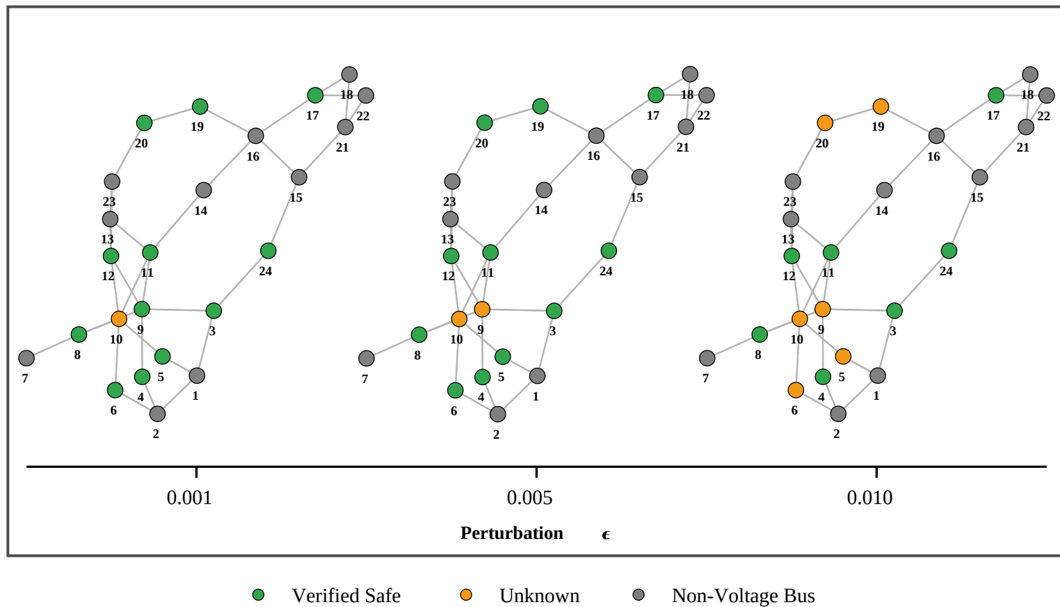
IEEE 24-Bus GINE ( —■— ) Verification
