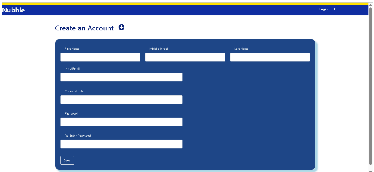
Figure 3.5.2: Registration Module
