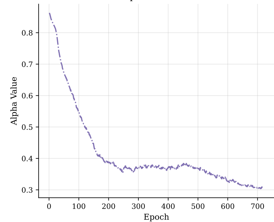
Alpha Evolution
