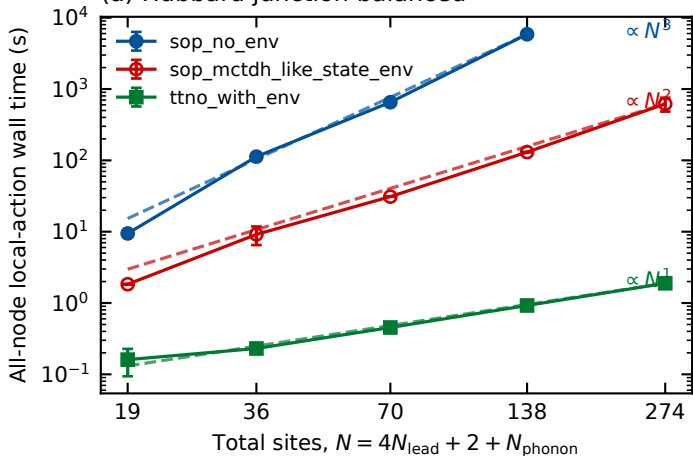
(a) Hubbard junction balanced
