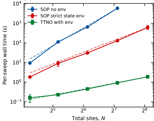
(a) Hubbard balanced
