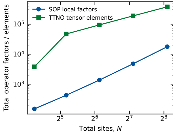
(b) SOP factors vs TTNO elements
