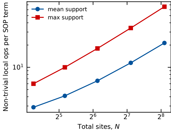
(a) SOP term support
