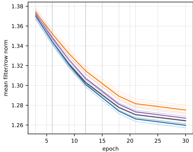
Weight norms at the temporal checkpoints (thin lines = seeds)
