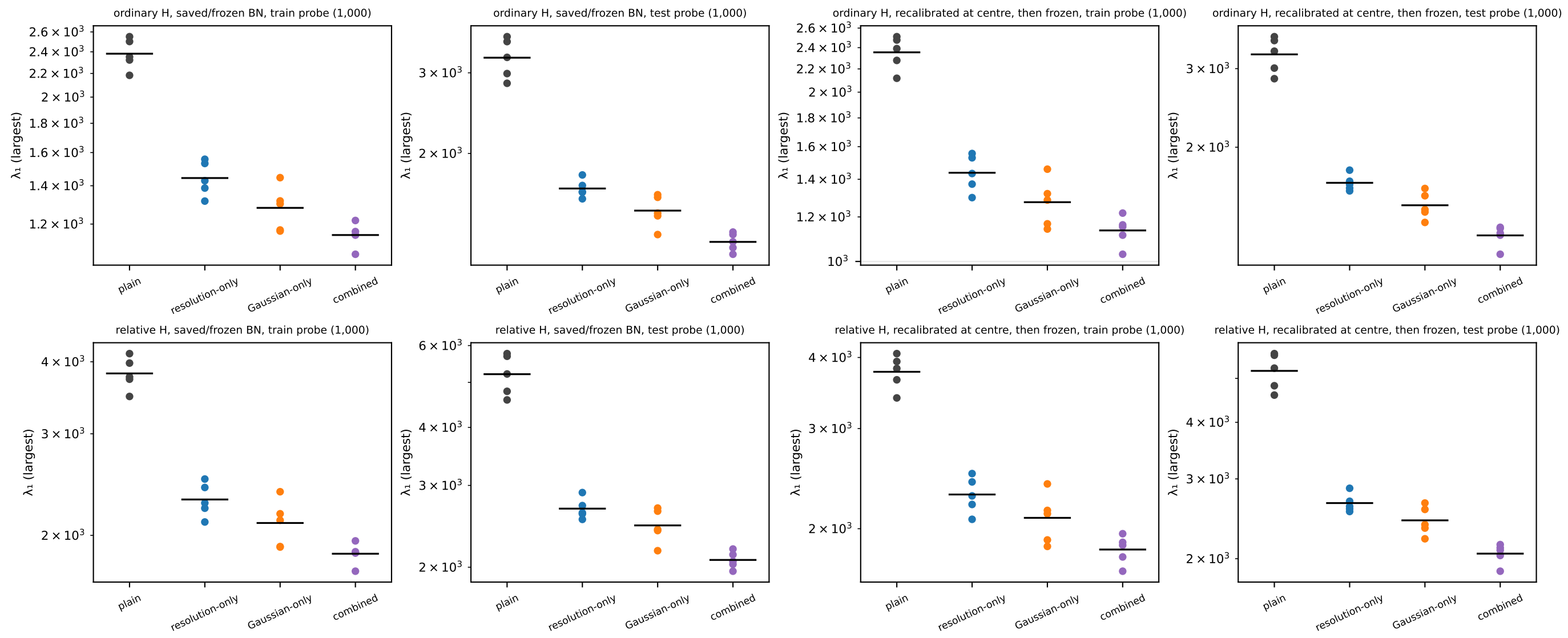
Hessian restricted to conv + fc weights at the epoch-30 solutions (dots = seeds, bar = mean; × = unconverged Ritz value)
