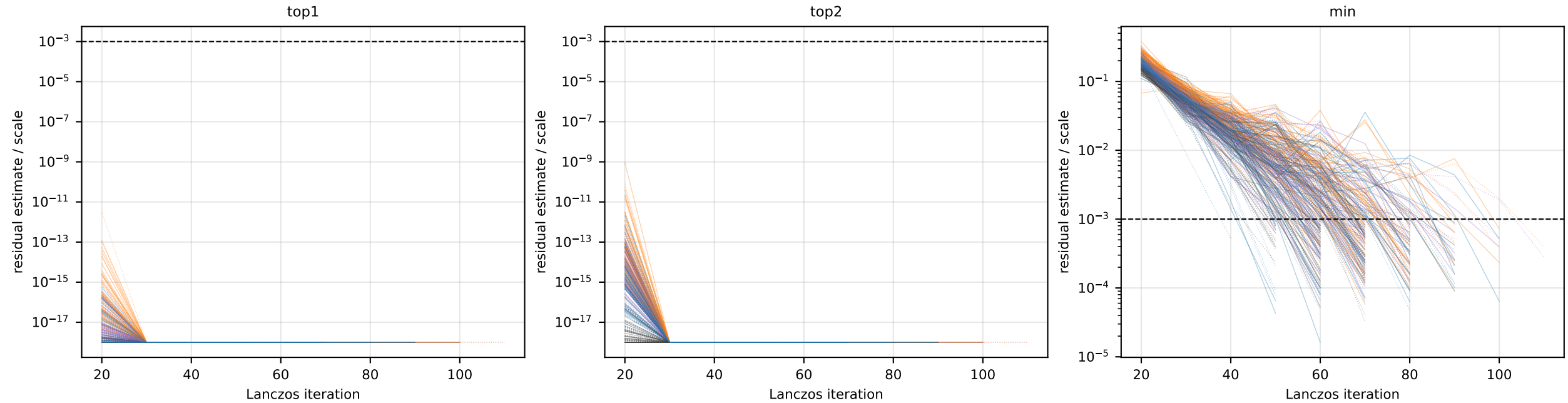
Convergence histories of all eigenproblems (solid = start 0, dotted = start 1; dashed = tolerance)
