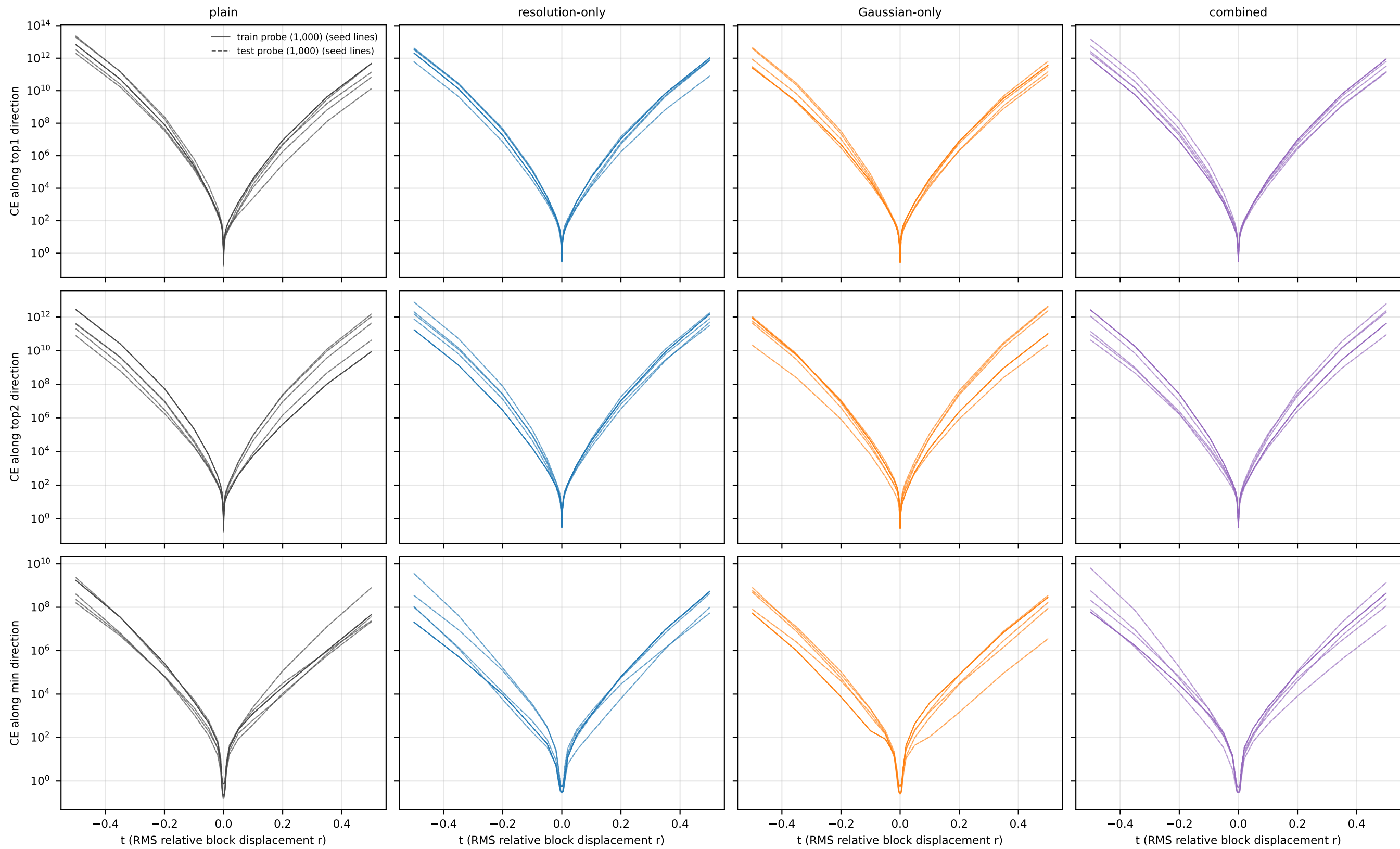
Cuts along relative-coordinate Hessian eigendirections (train-probe Hessian, recalibrated at centre, then frozen; evaluated under the same BN policy)
