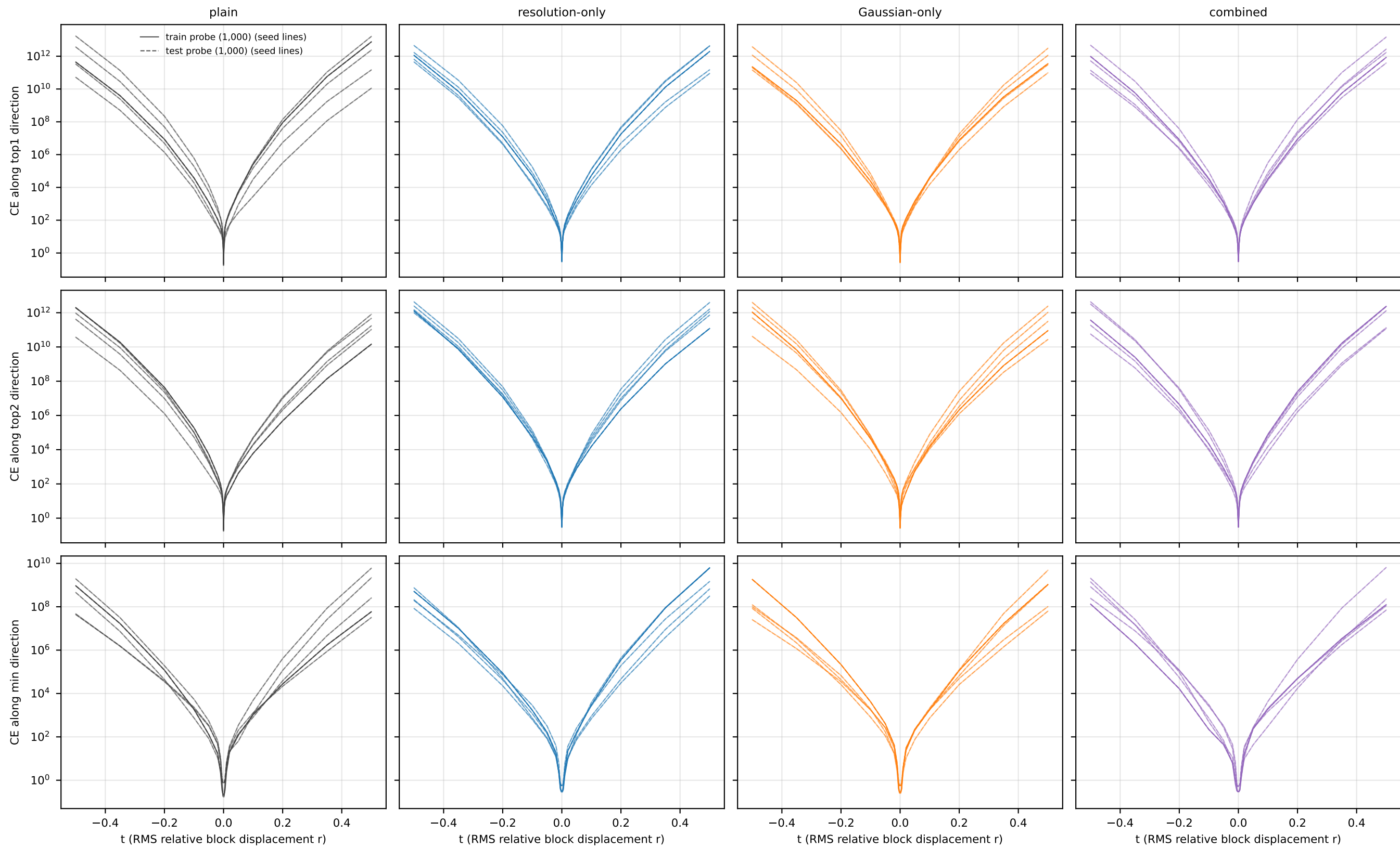
Cuts along relative-coordinate Hessian eigendirections (train-probe Hessian, saved/frozen BN; evaluated under the same BN policy)
