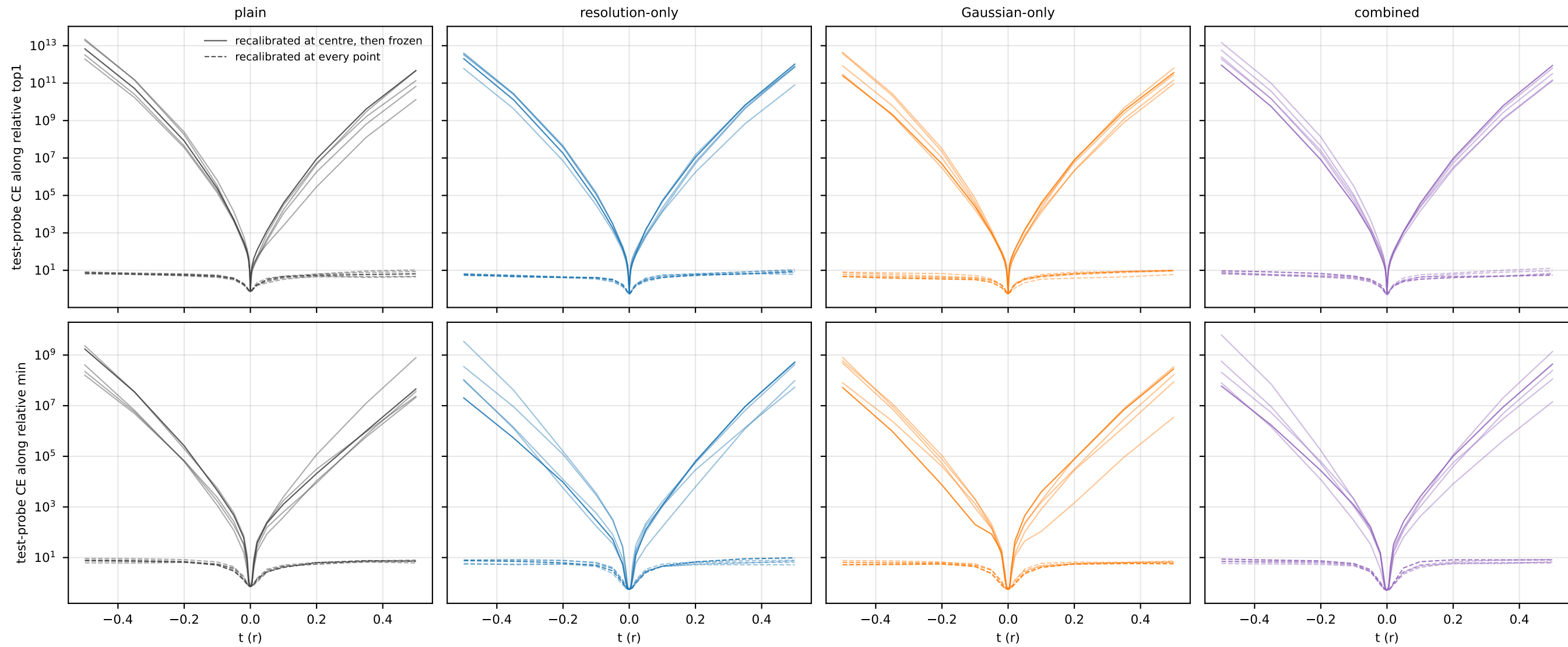
Same eigendirections (centre-frozen train-probe Hessian): frozen statistics vs recalibration at every point
