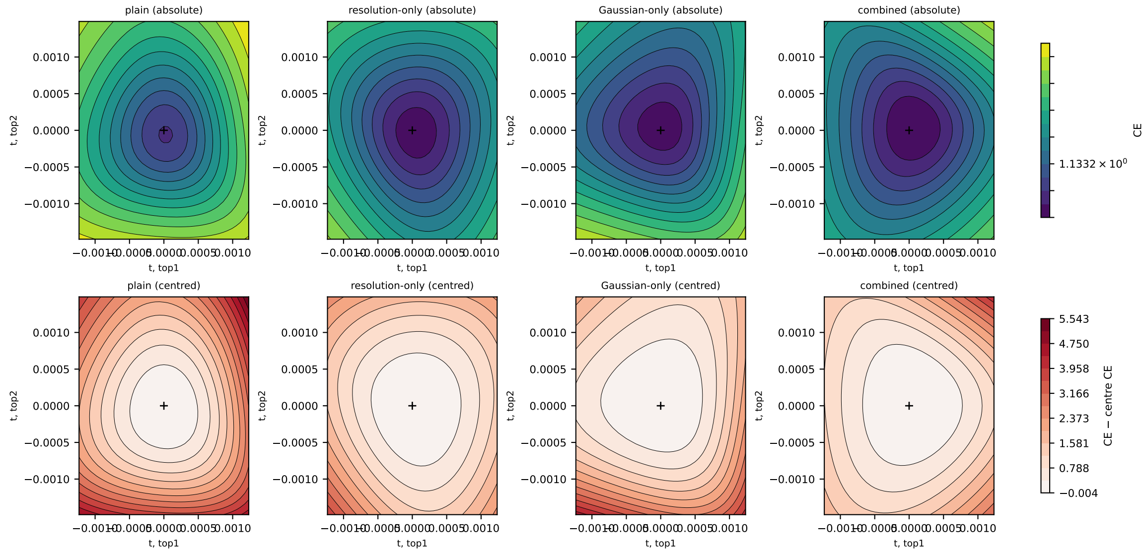
Seed 0 Hessian-eigendirection plane top1/top2, saved/frozen BN, test probe (1,000) (contours)
