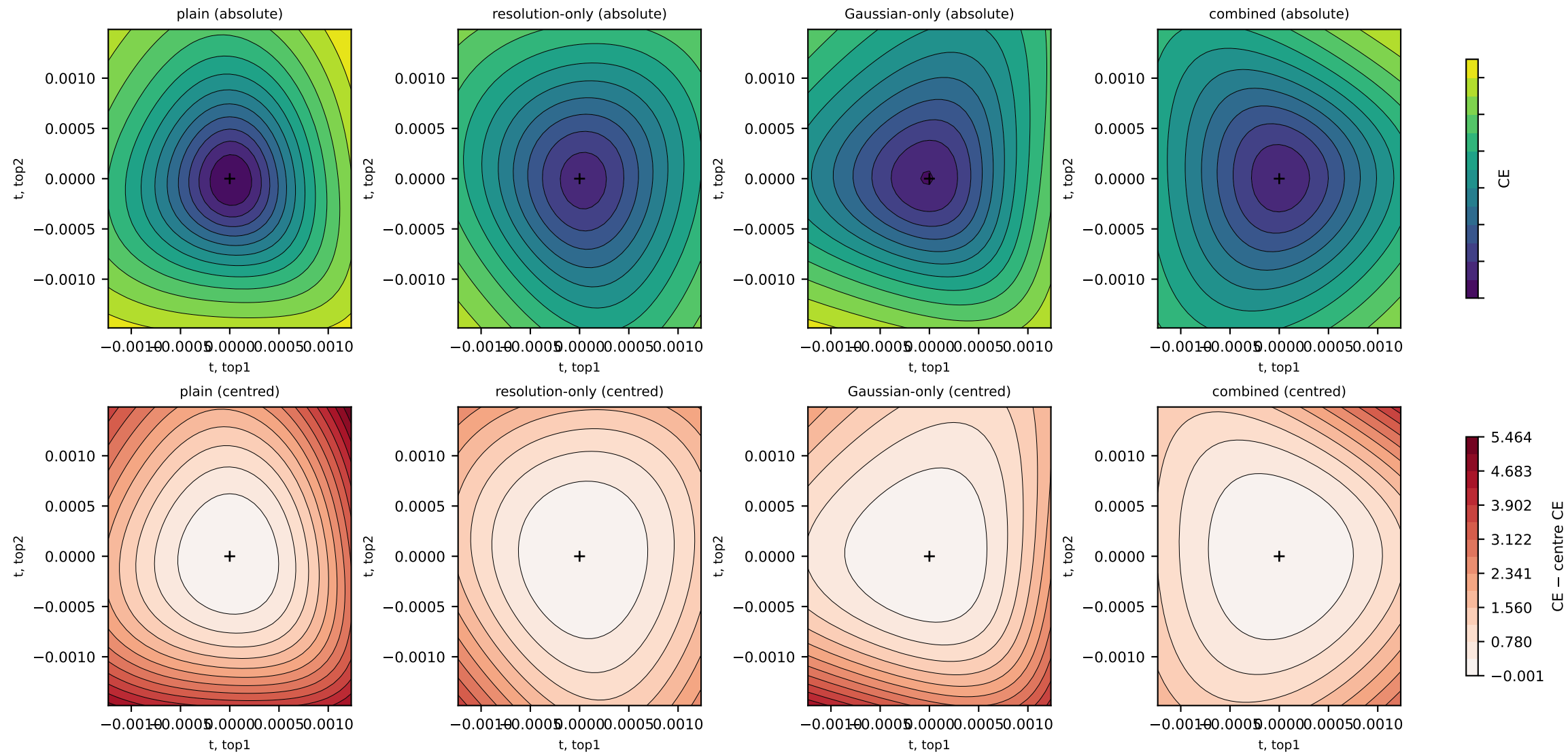
Seed 0 Hessian-eigendirection plane top1/top2, saved/frozen BN, train probe (1,000) (contours)
