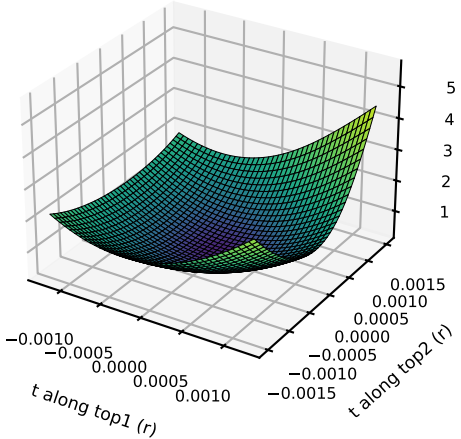
combined, seed 0 (centred)
