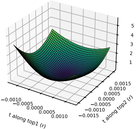
resolution-only, seed 0 (centred)
