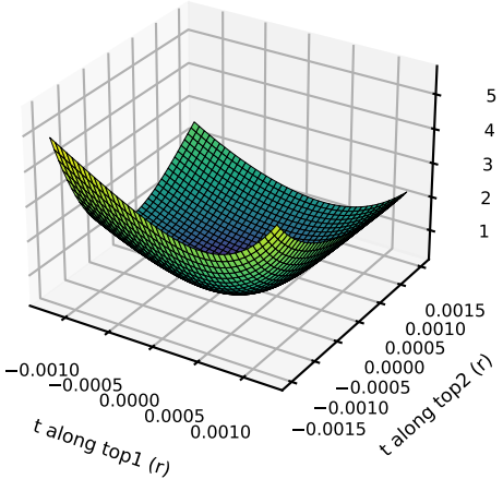
Gaussian-only, seed 0 (centred)
