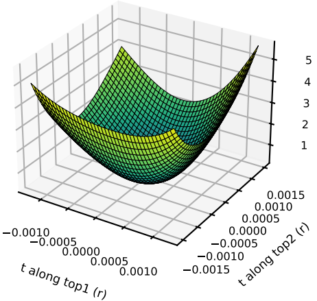
plain, seed 0 (centred)
