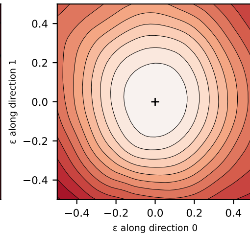
combined, seed 0
