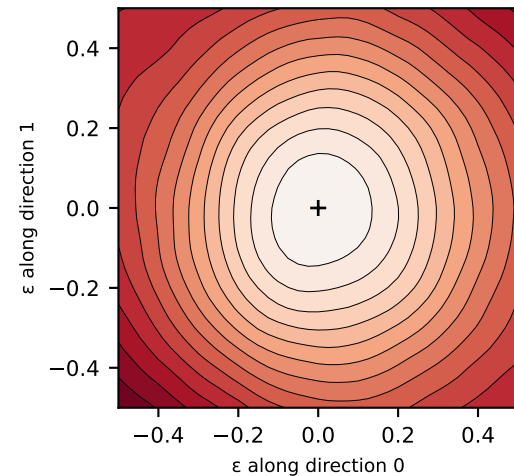
plain, seed 0
