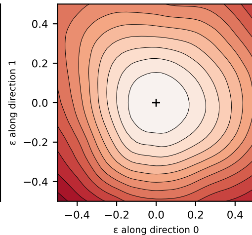
resolution-only, seed 0
