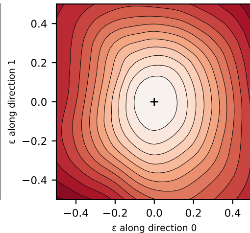
Gaussian-only, seed 0
