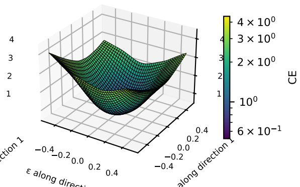
combined, seed 0
