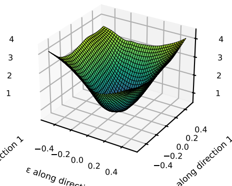
Gaussian-only, seed 0
