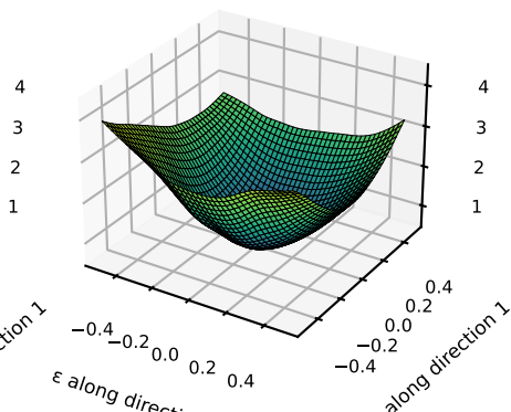
resolution-only, seed 0
