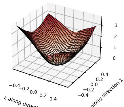
plain, seed 0
