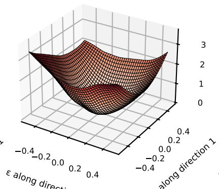
resolution-only, seed 0
