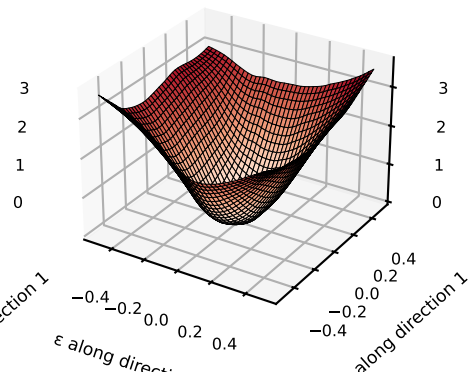
Gaussian-only, seed 0
