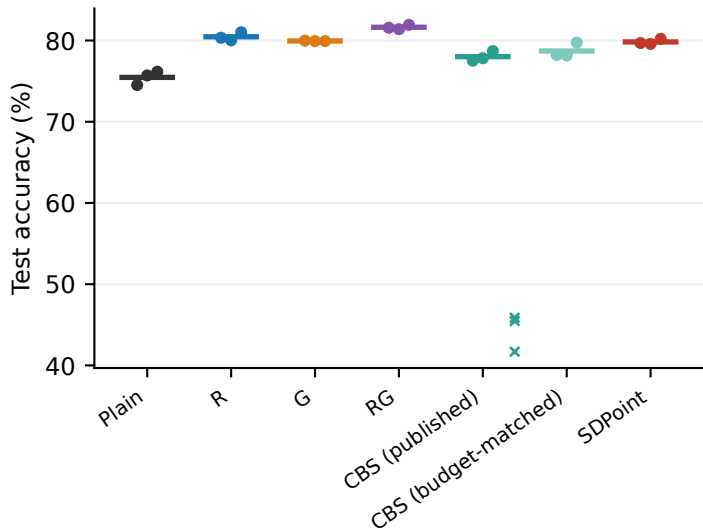
SGD (lr 0.005)
