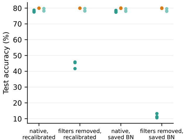
SGD (lr 0.005)
