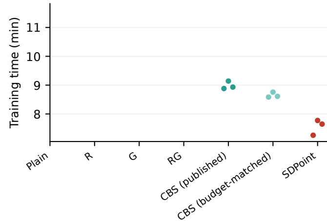
SGD (lr 0.005)
