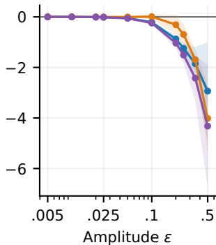
Saved / test
