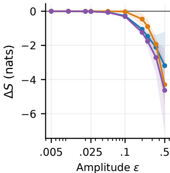
Saved / train
