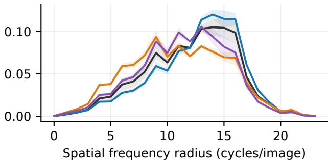
Input-Jacobian spectrum
