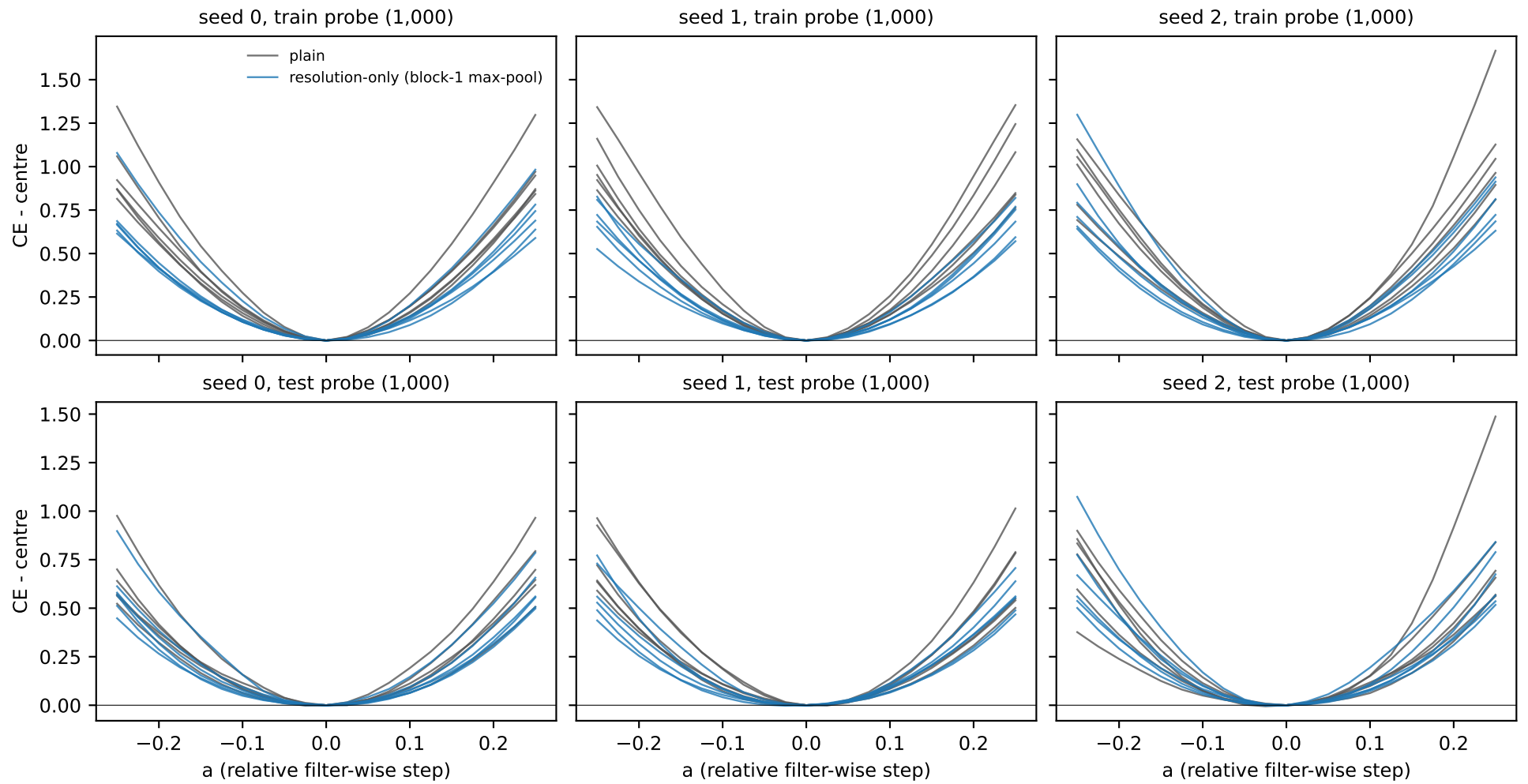
Robustness: 1-D slices along 6 filter-normalised directions per solution (pairs 0-4 axis D, pair 0 axis E), epoch 30, target state, recalibrated BN
