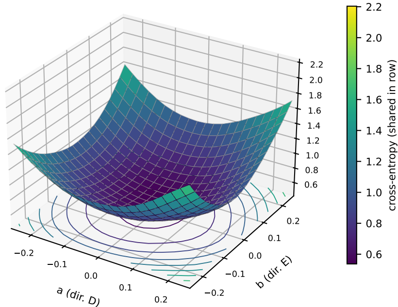
resolution-only, epoch 30, seed 0 test probe (1,000 imgs), centre CE 0.537
