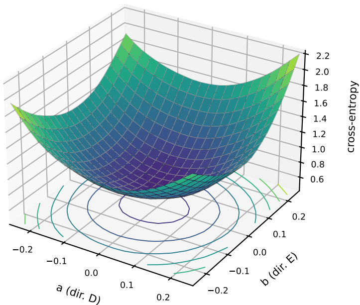
plain, epoch 30, seed 0 test probe (1,000 imgs), centre CE 0.726
