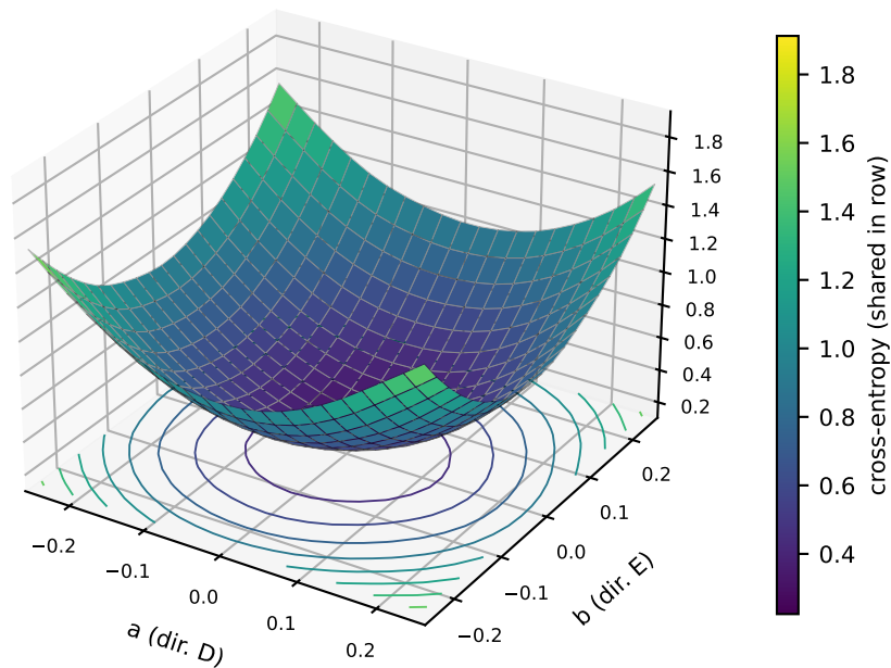
resolution-only, epoch 30, seed 0 test probe (1,000 imgs), centre CE 0.537
